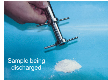
Standard Slot Sampler (without Bottle Holder)
